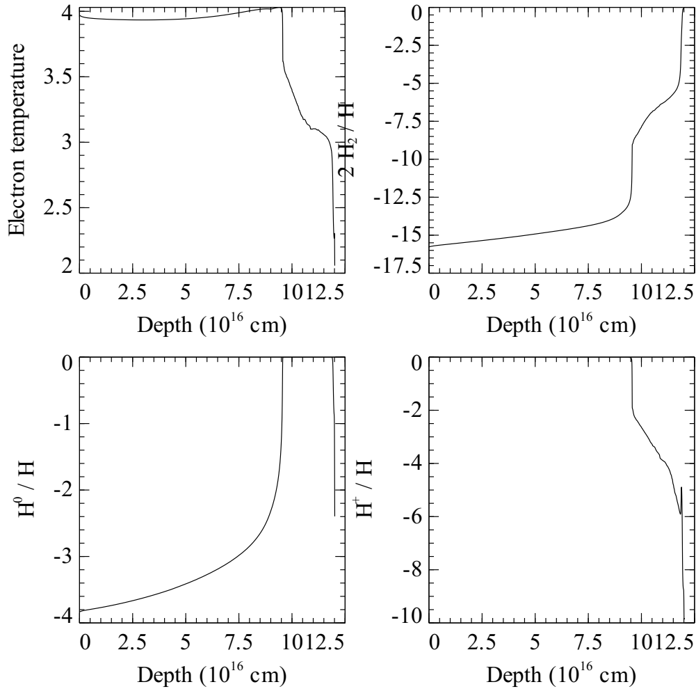
Figure 9: The electron kinetic temperature, and fractions of H in \text{H}_2 , \text{H}^0 , and \text{H}^+ , are shown as a function of depth into the Orion H II region / PDR.
