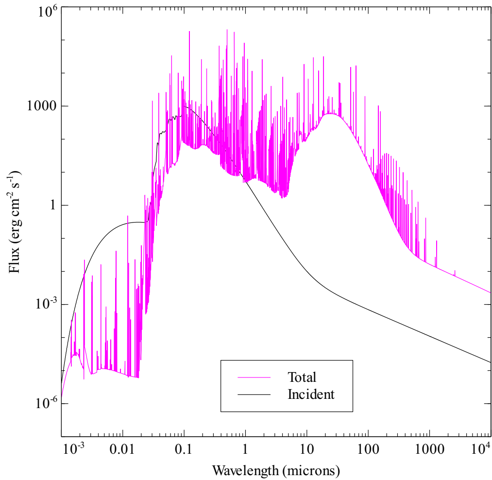
Figure 5: The incident (smooth) and emitted spectrum contained in the orion_hii_pdr_pp.con file. The x-axis is the wavelength in microns and the y-axis gives \nu f_\nu [erg cm -2 s -1 ]. This is produced by the save continuum command.
